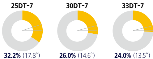
Max. Gradeability(Loaded)
